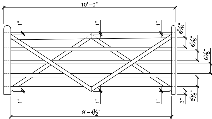
GATE DIMENSIONS
