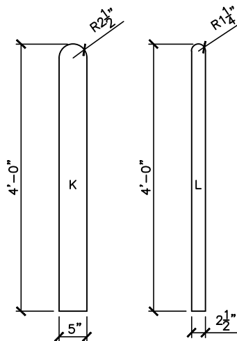
1-1" BOARD
