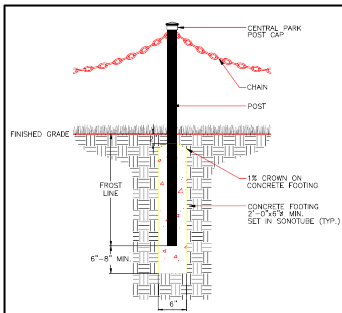
Central Park Post Installation Detail
