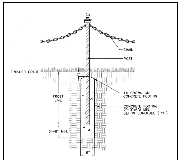
Boston Garden Post Installation Detail
