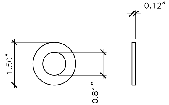
WASHER X2
