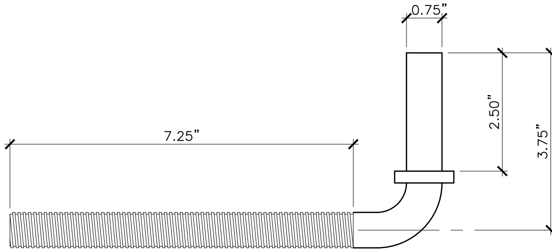
SIDE
