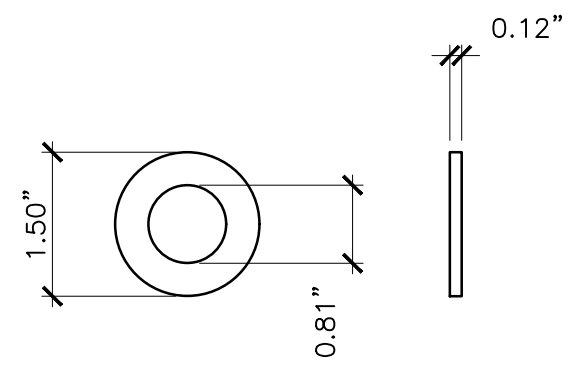
WASHER X2
